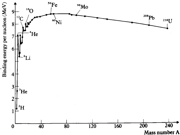
14.9 The binding energy per nucleon as a function of mass number A .
